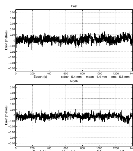
Fig. 20 Master Time-Loc : Locata receiver East and North static positioning error.
