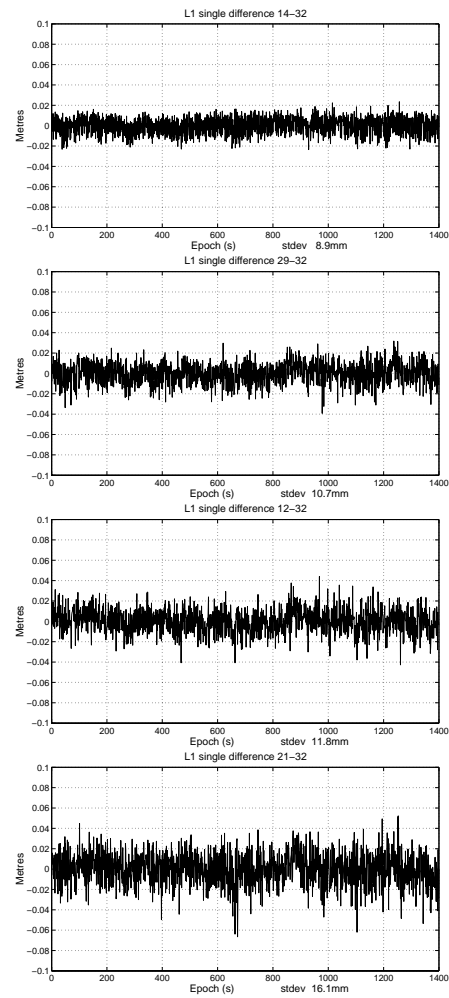
Fig. 19 Cascaded Time-Loc : LocataLite single-differences using 32 as reference (14, 29, 12, 21, top to bottom).
