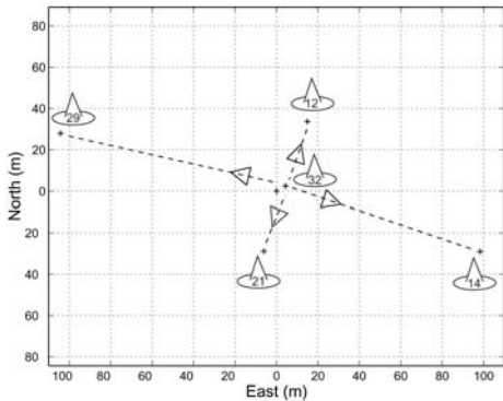
Fig. 15 Master Time-Loc procedure using ‘master’ LocataLite 32.
