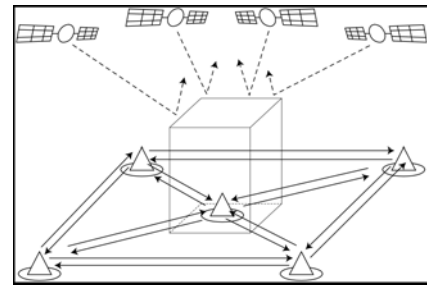
Fig. 10 Propagating the LocataNet indoors.
