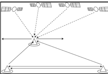
Fig. 7 Establishing a LocataNet , step 3.
