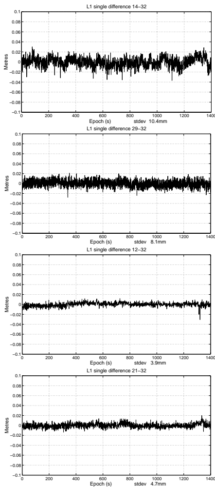
Fig. 18 Master Time-Loc : LocataLite single-differences using 32 as reference (14, 29, 12, 21, top to bottom).
