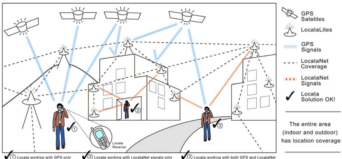
Fig. 2 The Locata technology positioning concept.
