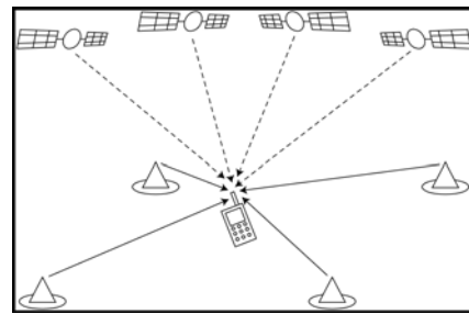
Fig. 11 Positioning outside using LocataNet and GPS.
