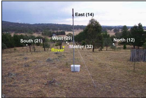
Fig. 14 Outdoor experimental LocataNet comprised of five LocataLites .
