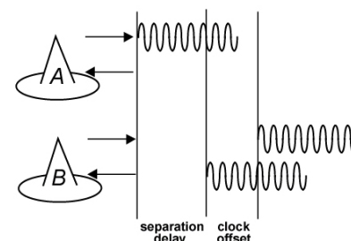
Step 3. LocataLite B transmits a unique signal.
