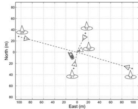
Fig. 17 Locata receiver positioning using LocataNet signals from either Master or Cascaded Time-Loc .
