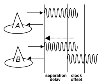
Step 6. LocataLite B corrects for A & B separation.
