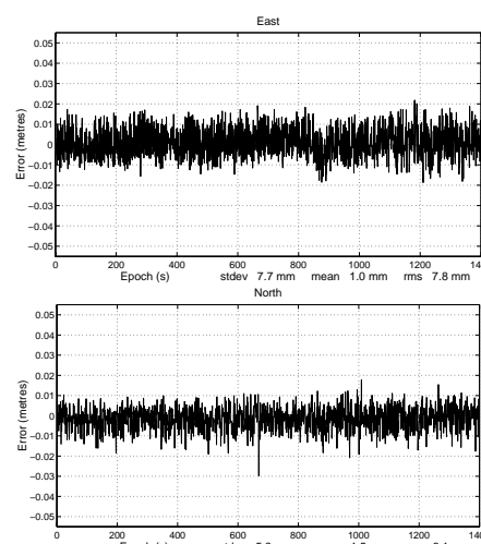
Fig. 21 Cascaded Time-Loc : Locata East and North static positioning error.
