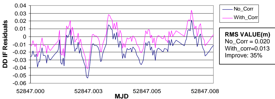
Fig. 11 DD IF residuals (m) of Satellite pair PRN26-30
