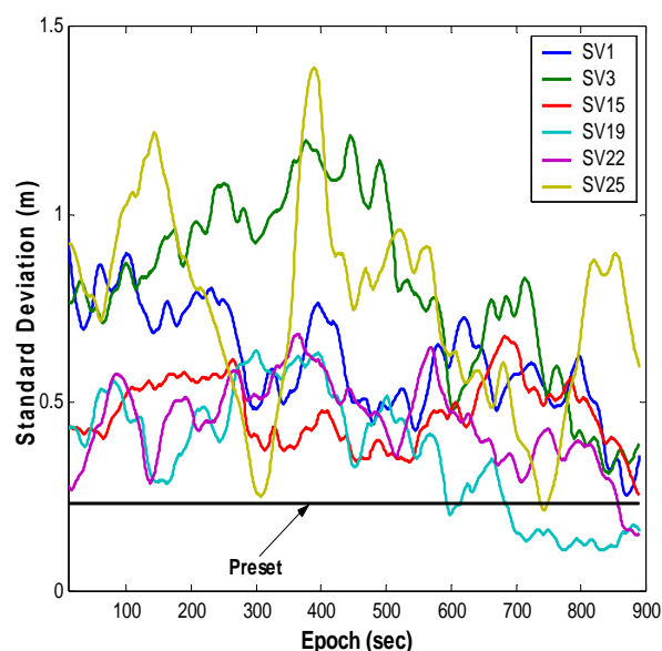
Fig. 7 Standard deviation of C1 pseudo-range measurements
