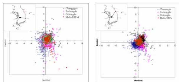
Fig. 9 Multi-Ref.s DGPS positioning accuracy; 1.164 m (left) and 0.788m (right)
