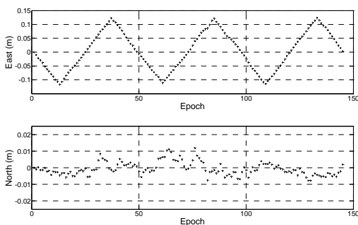
Fig. 13 Mean static East and North time series: GPS
